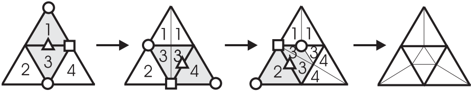
Figure 6: Generating an adaptive 1-to-4 subdivision split with three successive vertex split operations. The support of all quarks contains exactly two different triangle indices (b-quarks).
